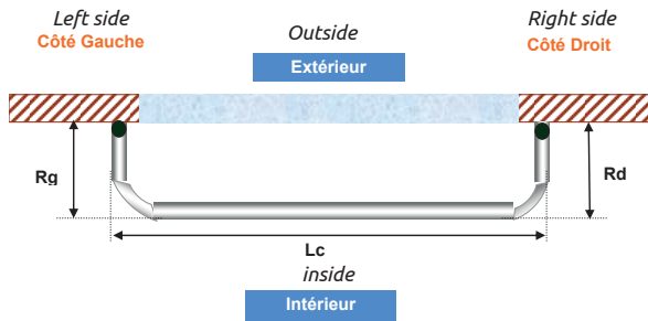
KS rail – 2 angles of 90°: 1 or 2 curtains
