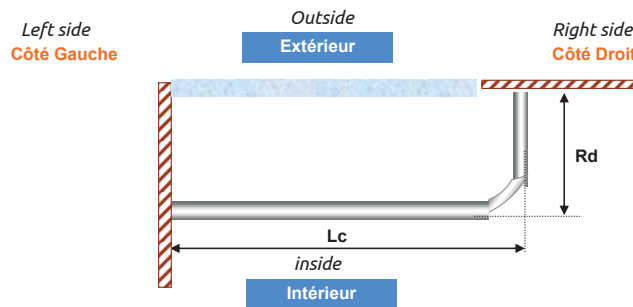
KS rail (BL) – 1 angle of 90° (Right side): 1 Curtain
