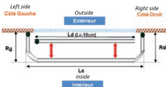
KS rail – 2 angles of 90°: 1 or 2 curtains + sheer
