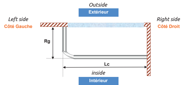
KS rail (BL) – 1 angle of 90° (Left side): 1 Curtain
