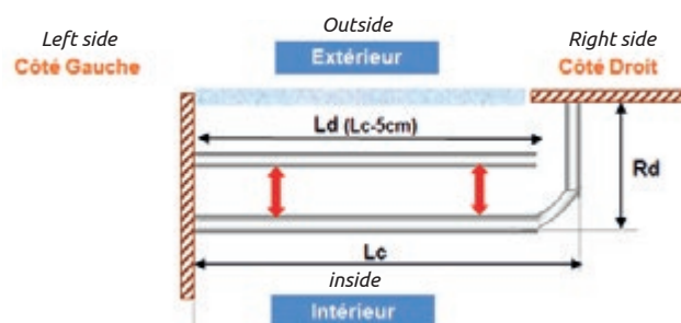
KS rail (BL) – 1 angle of 90° (Right side): 1 Curtain + sheer
